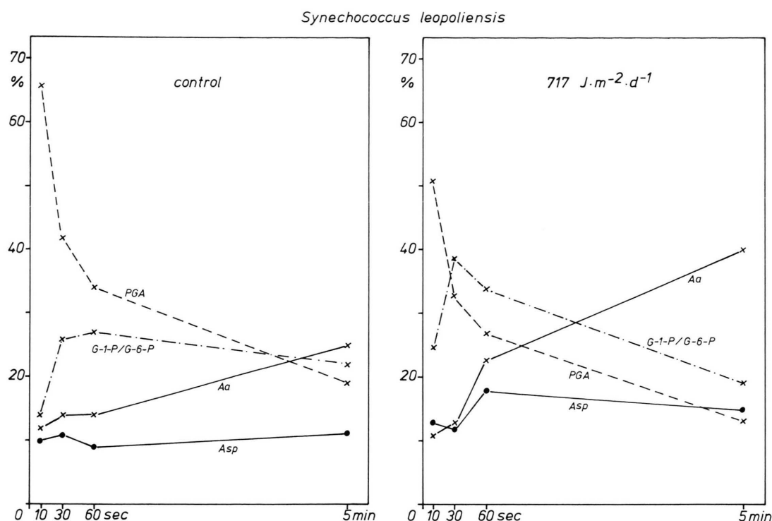
Fig. 4. Effect of UV-B radiation ( 717 \text{ J m}^{-2} \text{ d}^{-1} , weighted) on time course of ^{14}\text{C} -incorporation into various soluble photosynthetic products (% distribution of total ^{14}\text{C} -labelled compounds) of Synechococcus leopoliensis . For abbreviations and more details see Fig. 3 and Materials and Methods.
