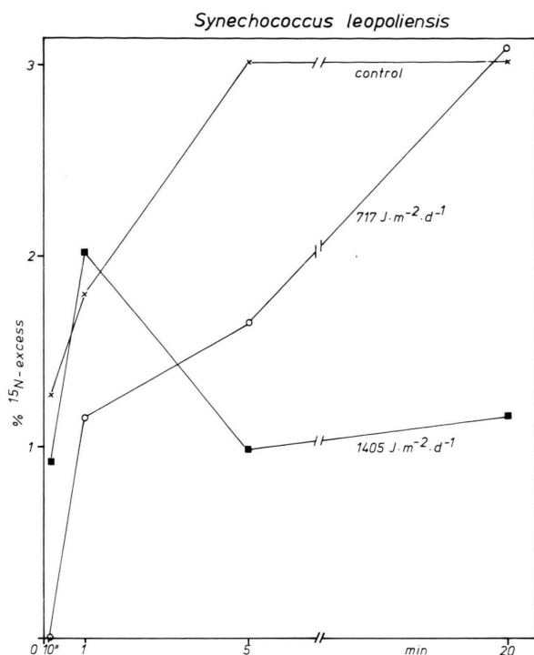
Fig. 1. Effect of UV-B radiation (717 and 1405 J m -2 d -1 , weighted) on uptake of 15 N-nitrate (K 15 NO 3 , 96 atom %; 1 mM final concentration in the suspension) of Synechococcus leopoliensis . After UV-B exposure cells were resuspended in a nitrogen-free nutrient medium; 15 N-nitrate was added under steady state conditions after 15 min photosynthesis. The data represent the percentage of 15 N of the total nitrogen content. For further details see Materials and Methods.
